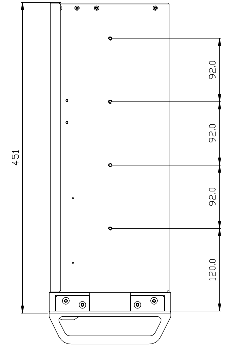
Right-side View
